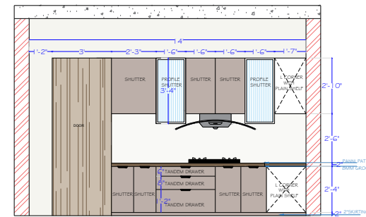
WALL ELEVATION B
