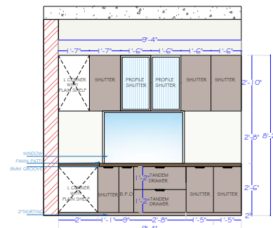
9-4 WALL ELEVATION C
