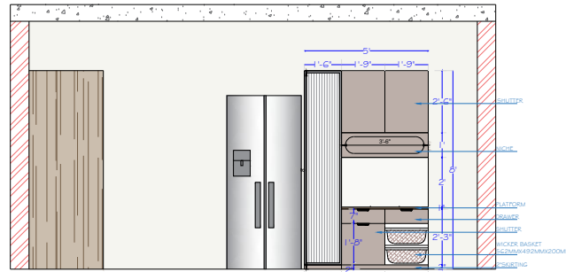
WALL ELEVATION A
